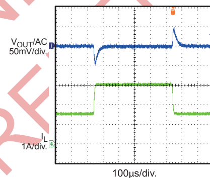
Load Transient Response I_{OUT} = 1.5A-3A
