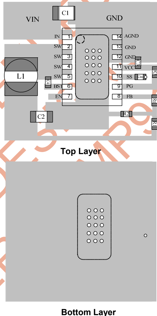
Figure 7—PCB Layout
