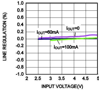
Line Regulation
