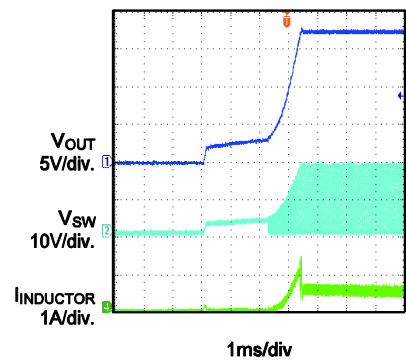
Startup IOUT=100mA
