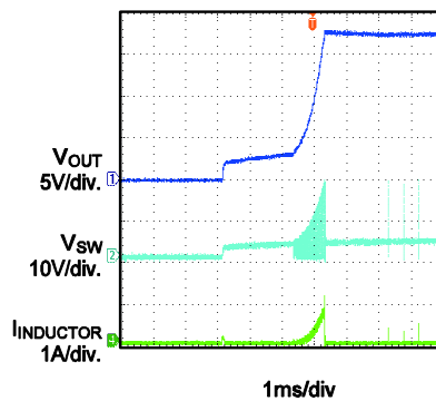
Startup IOUT=0
