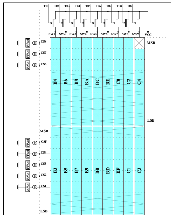
Figure 11 Open/Short Register
