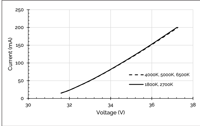
Figure 1: Forward Voltage vs. Forward Current, T_c=25^\circ\text{C}
