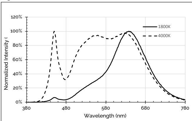
Figure 18: 1800K - 4000K with 90 CRI
