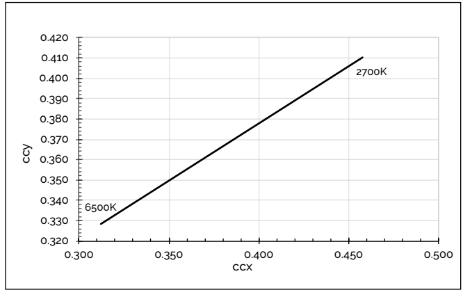
Figure 12: CCT Tuning Range, Tc=85
