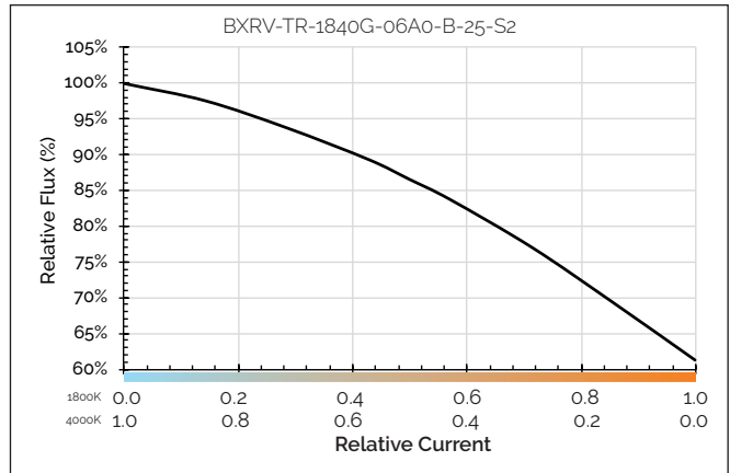
Figure 10: Relative Flux vs. Relative Current
