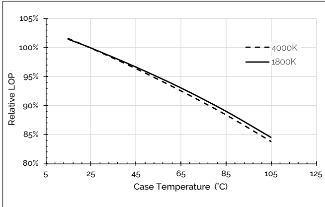
Figure 5: Relative Light Output vs. Case Temperature
