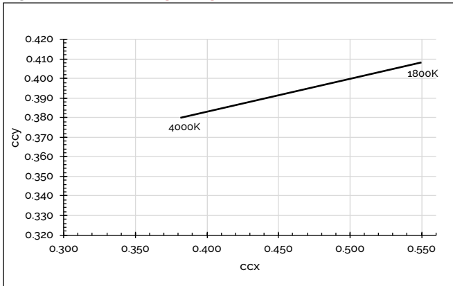
Figure 13: CCT Tuning Range, Tc=85
