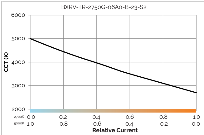
Figure 6: CCT vs. Relative Warm White Current
