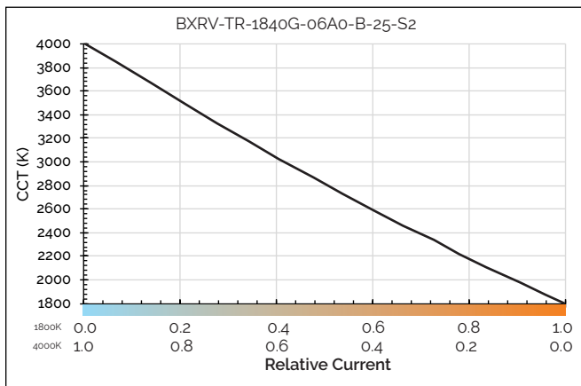
Figure 8: CCT vs. Relative Current, Tc=85C
