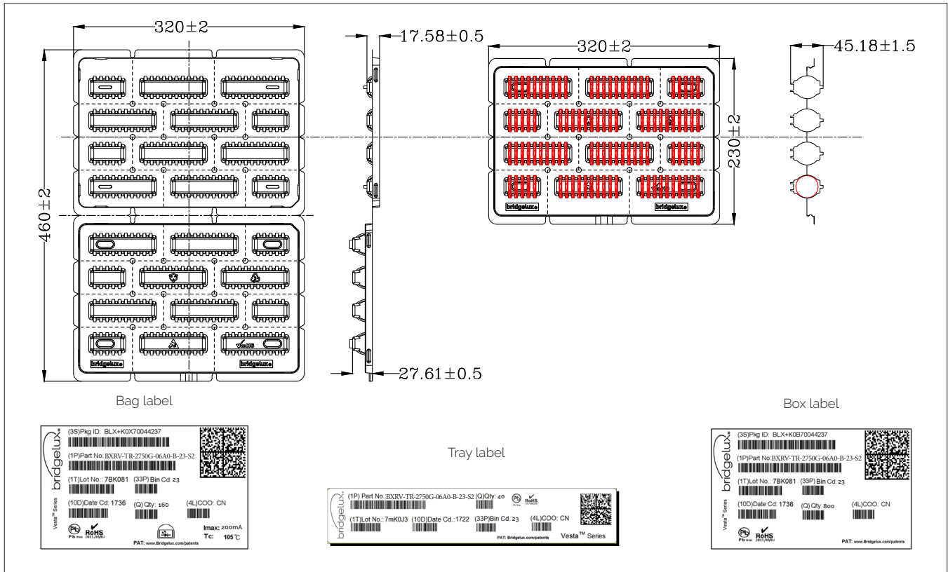
Figure 22: Packaging Specifications
