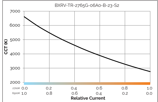
Figure 7: CCT vs. Relative Warm White Current
