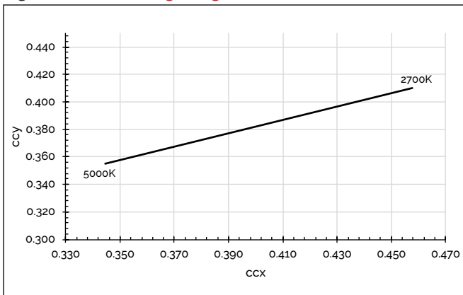
Figure 11: CCT Tuning Range, Tc=85
