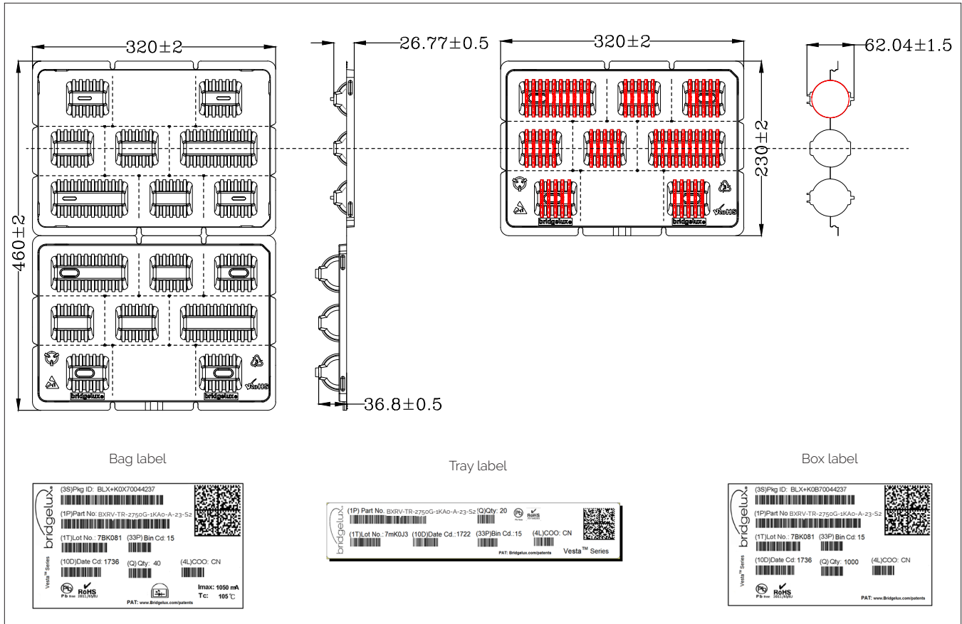
Figure 17: Packaging Specifications
