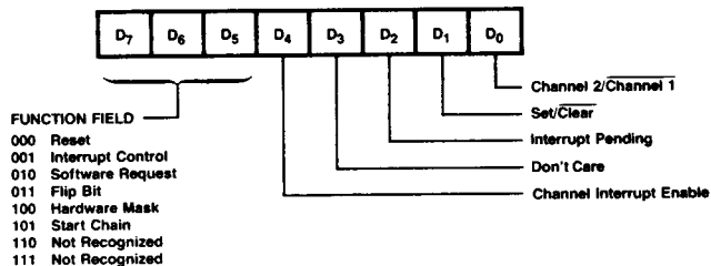
Figure 19. Command Register
