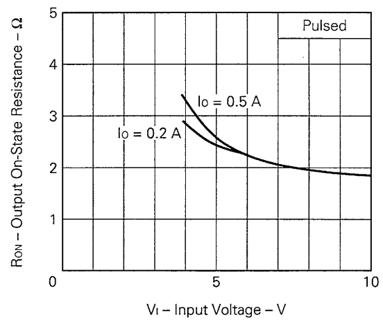
R_{ON} - V_i Characteristic
