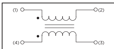
equivalent circuit
