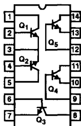
HFA3046 TOP VIEW
