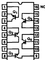
HFA3096 TOP VIEW
