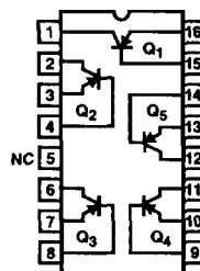
HFA3128 TOP VIEW
