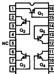
HFA3127 TOP VIEW
