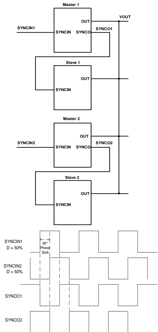
Figure 8: Four-Phase Configuration
