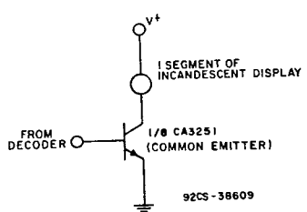
Fig. 6 - Schematic diagram showing one transistor of the CA3251 driving one segment of an incandescent display.
