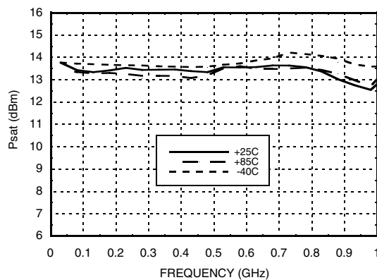
Psat vs. Temperature @ 3V
