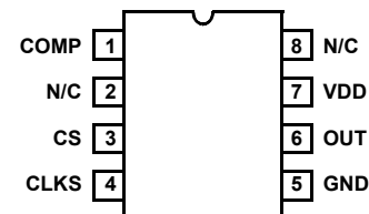
ISL6729 (8 LD SOIC, MSOP) TOP VIEW
