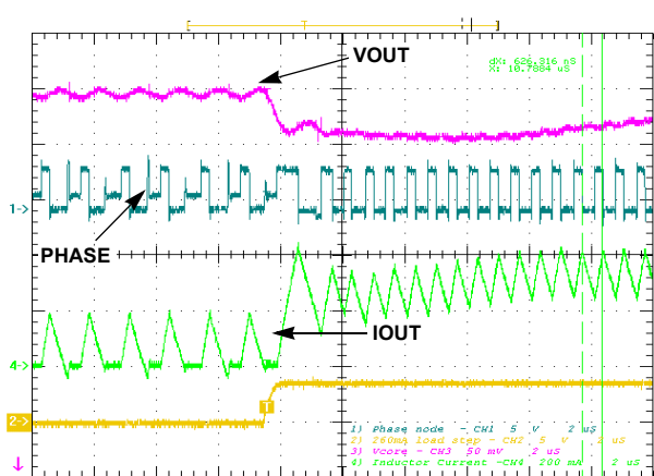
50mA to 260mA load step on VOUT. Top: Output voltage, 50mV/DIV; Phase node, 5V/DIV; Inductor current, 200mA/DIV, 2 \mu s/DIV
