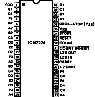
Figure 1: Pin Configuration
