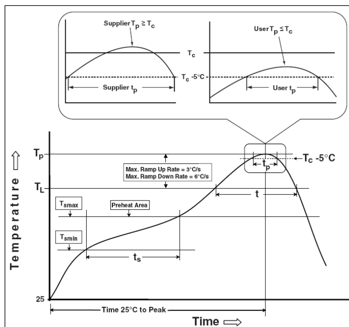
Figure 74 Classification Profile
