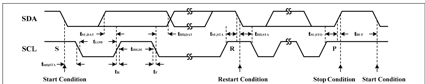
Figure 54 Interface Timing
