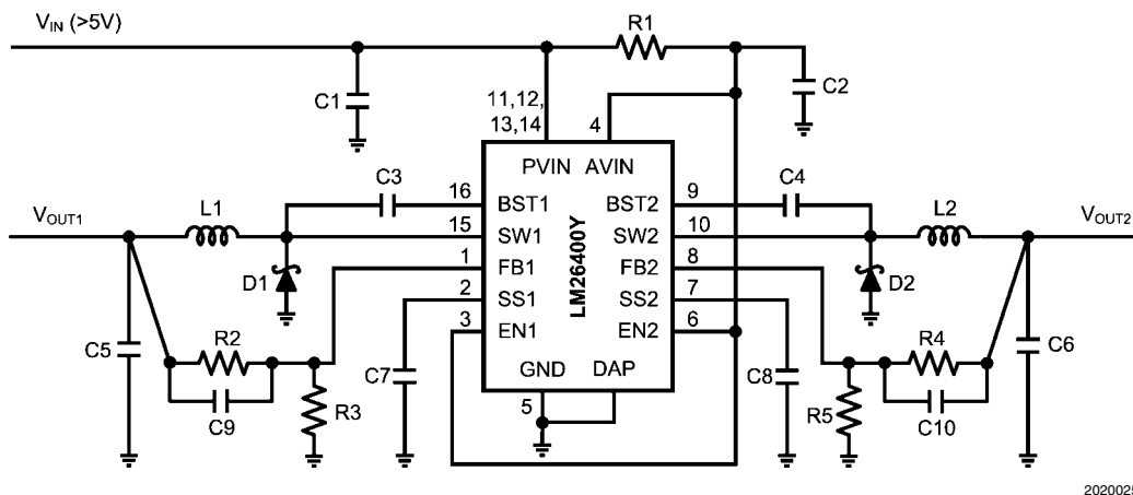
FIGURE 10. Example Circuit 1
