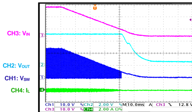
Shutdown through the Input Voltage
