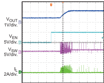
V_{OUT} Prebias Start Up
