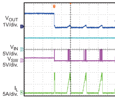
Hiccup With Output Short
