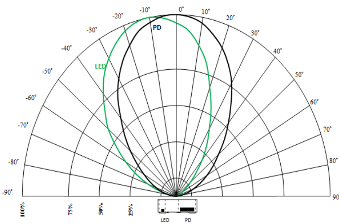
Directivity at Package direction X
