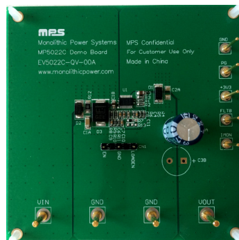
(L x W x H) 8.55cm x 8.55cm x 1.6mm
