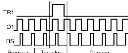
Figure 33: CIS TR1 Timing Mode 1
