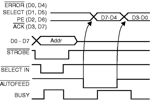
Figure 55: Reading from the Configuration Register (Nibble Mode)
