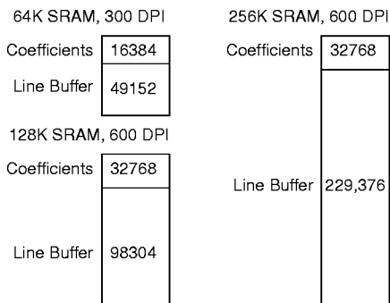
Figure 43: Typical Memory Maps for External SRAM
