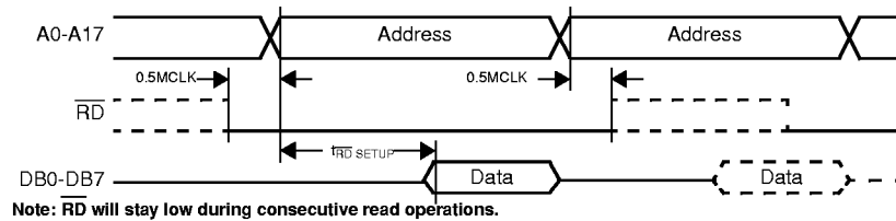
Figure 9: SRAM Read
