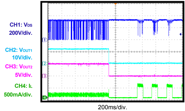
V_{OUT1} Short Circuit Full Load
