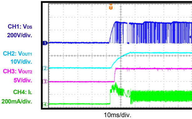
Start-Up Full Load
