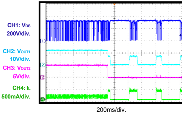
V_{OUT2} Short Circuit Full Load
