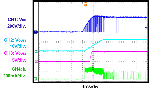
Start-Up No Load
