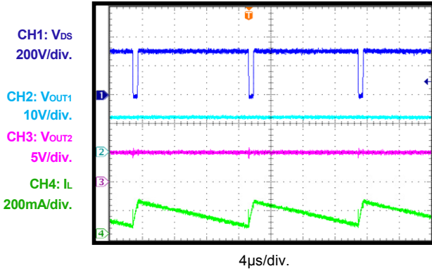
Normal Operation Full Load
