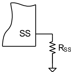
Figure 6: External Resistor for Sampling Time Customization
