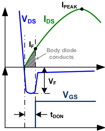
Figure 9: Turn-On Delay Affects Efficiency
