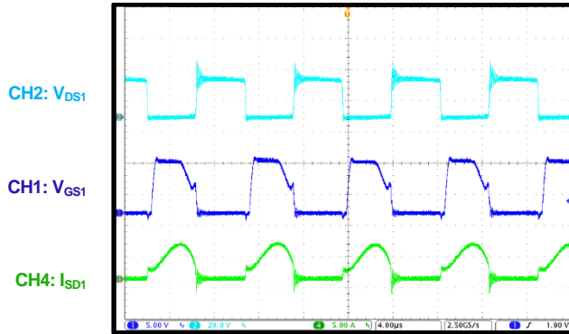
Operation in 180W LLC Converter
