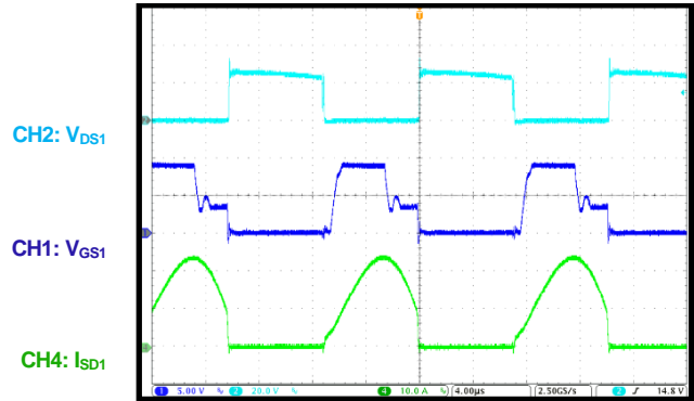
Operation in 180W LLC Converter
