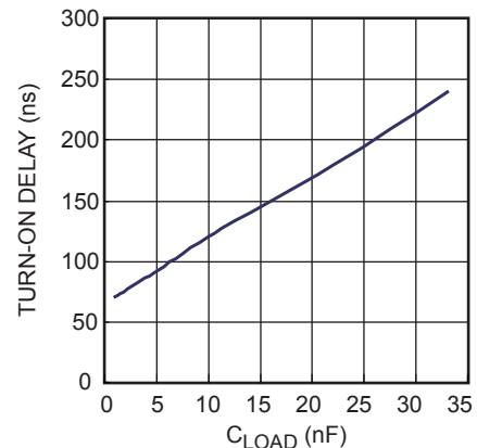
Figure 11: Turn-On Delay vs. C_{load}
