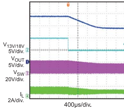
19V to 14V Switching I_{OUT} = 0.5A
