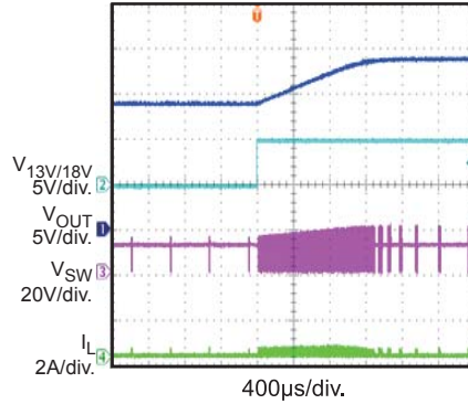
14V to 19V Switching I_{OUT} = 0A
