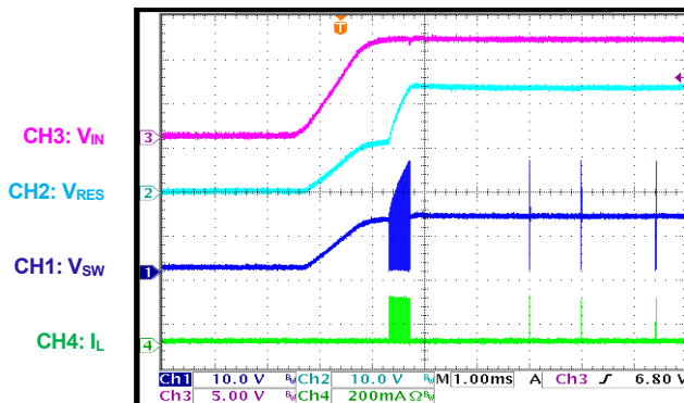
Start-Up through VIN (for Internal Boost) I_{OUT} = 0A
