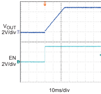
Turn on Delay and Rise Time Cdv/dt=1nF, C OUT =10uF, no load
