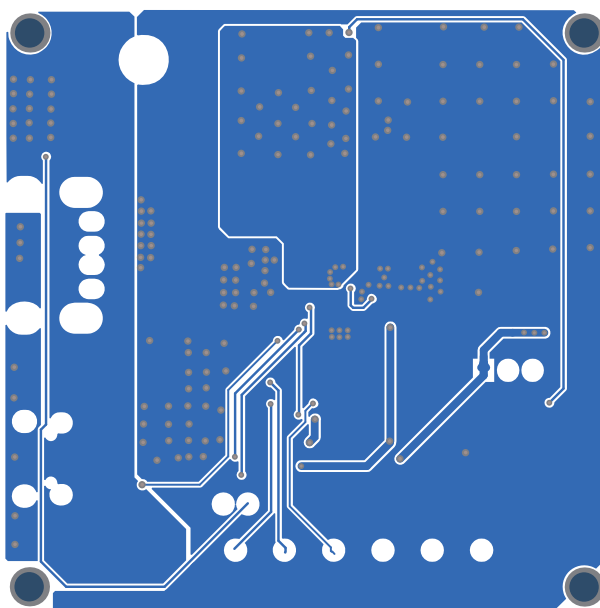
Figure 2: Bottom Layer
