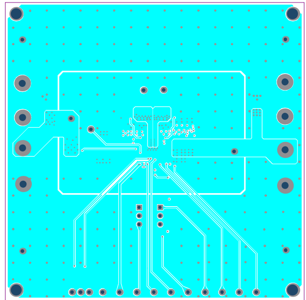
Figure 28: Mid-Layer 2
