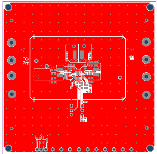
Figure 26: Top Layer
