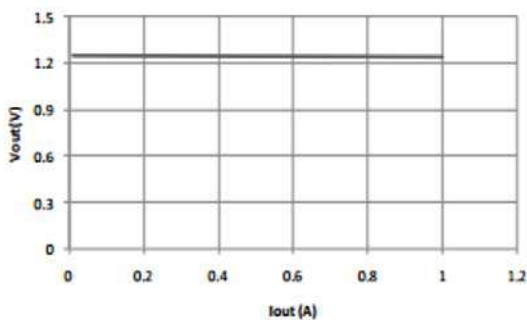
Load regulation ICW1117-ADJ Vout Vs. Iout
