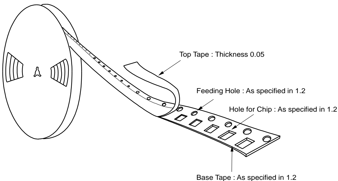
Fig3 Taping Diagram
