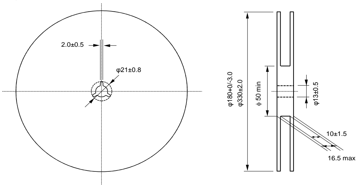
Fig3 Taping Diagram
