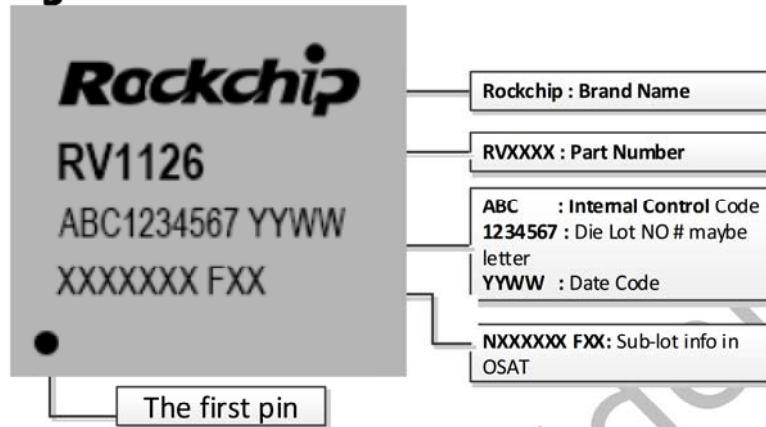
Fig.2-1 Package definition
