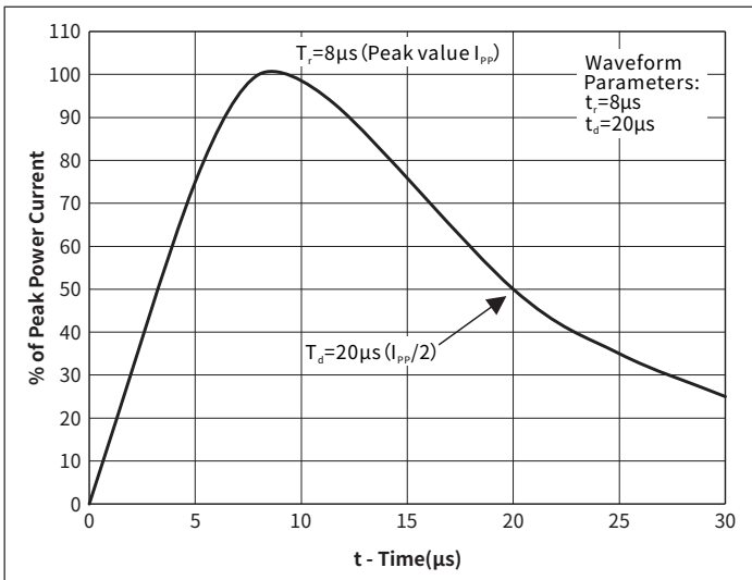
Fig.1 Pulse Waveform
