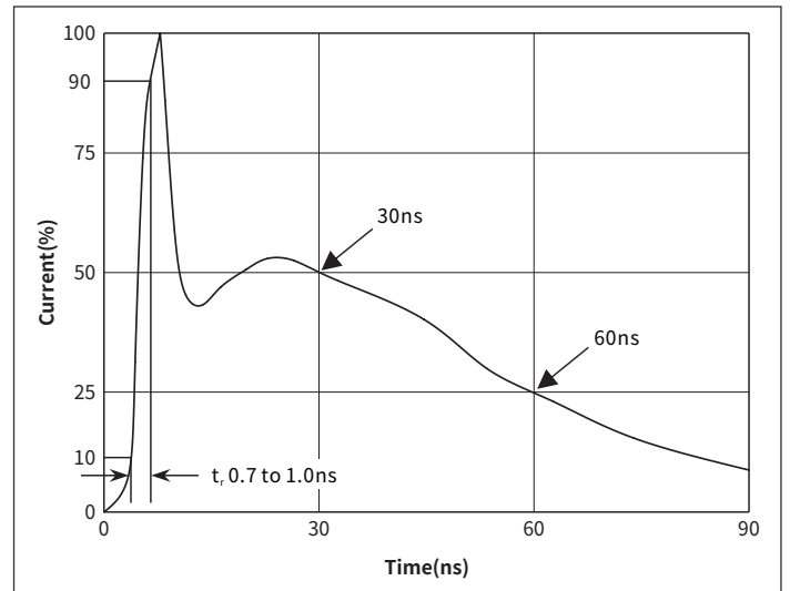
Fig.2 Pulse Waveform-ESD(IEC61000-4-2)
