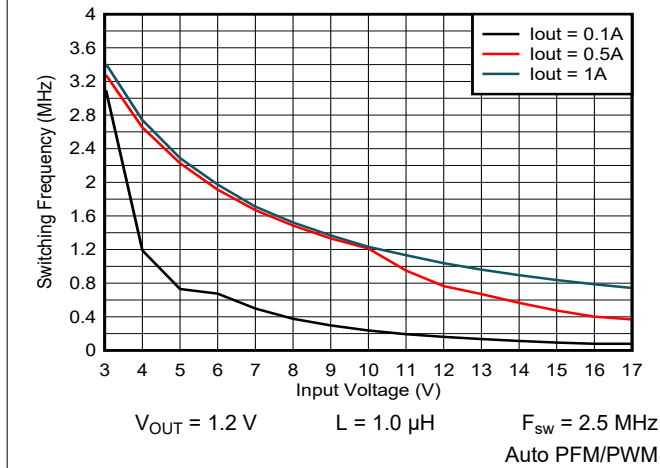
Figure 9-17. Switching Frequency vs Input Voltage
