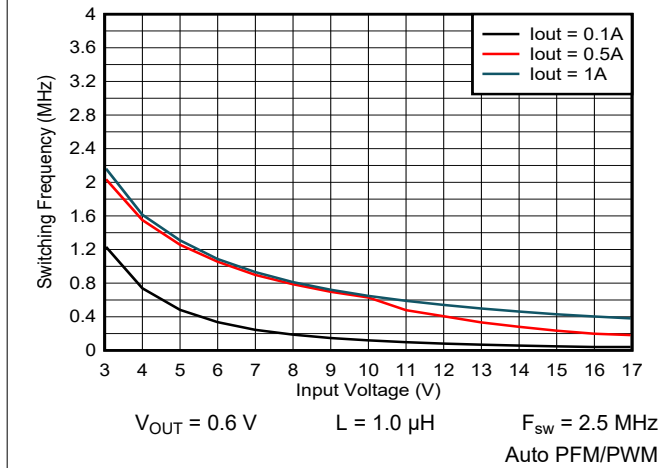
Figure 9-29. Switching Frequency vs Input Voltage
