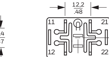
0.020 in x 0.110 in Termination
