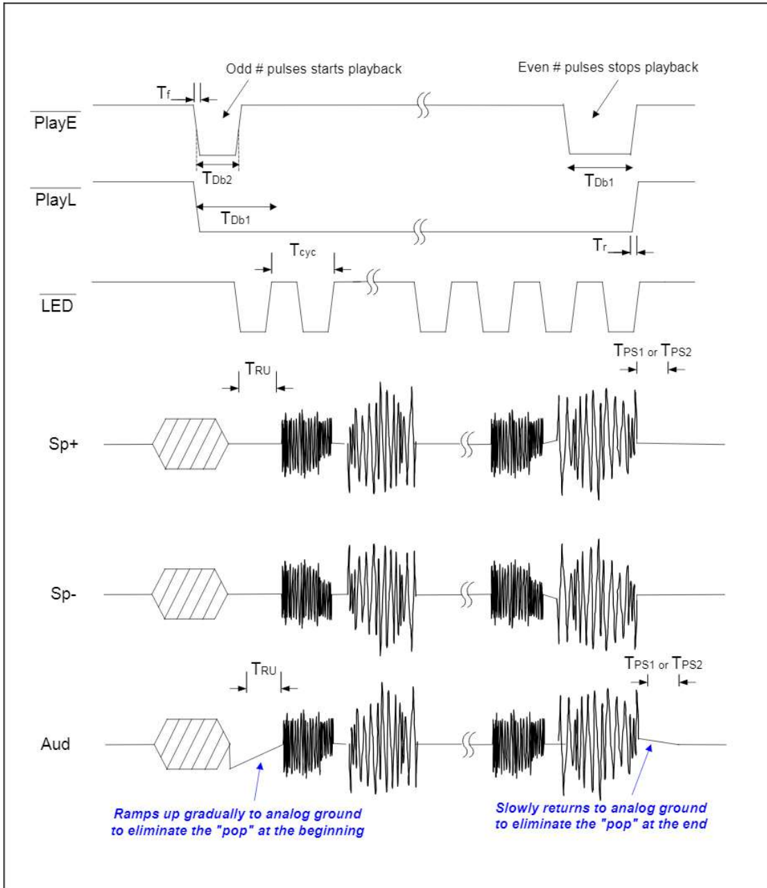
FIGURE 2: PLAYBACK OPERATION
