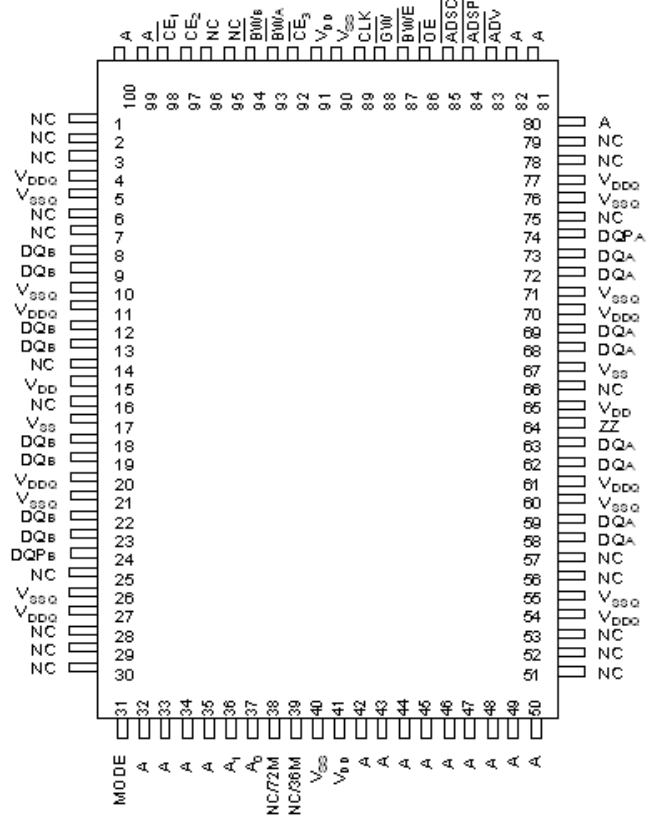
Figure 2. CY7C1382D, CY7C1382F (1M X 18)
