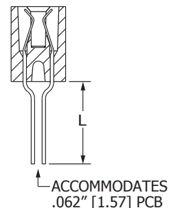
CARD EXTENDER (KR, KN)
