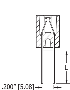
DIP SOLDER/WIRE WRAP (KS, KD, KM)
