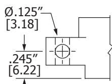
SIDE MOUNTING (S)
