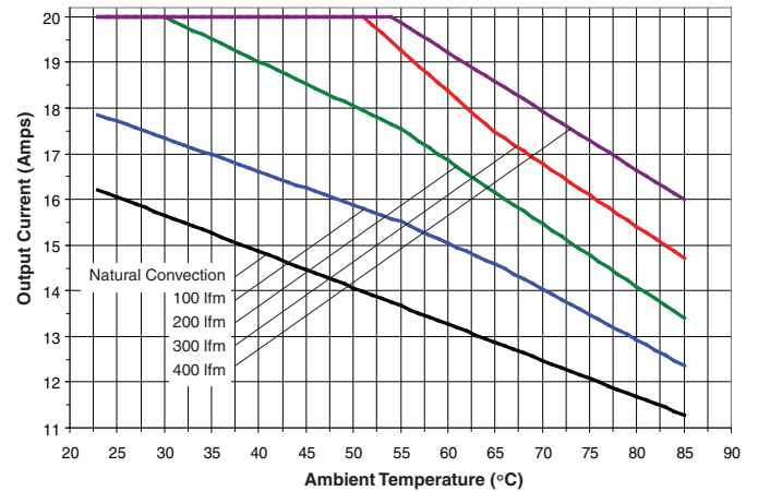
UQQ-5/20-Q48P Maximum Current Temperature Derating at sea level (VIN = 48V, with baseplate, transverse airflow)
