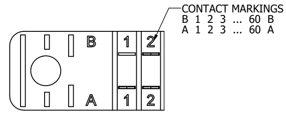
CONTACT ID SCALE 5:1
