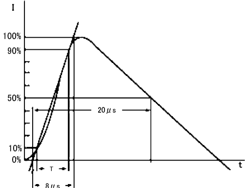
Fig. 6.2.2 Based on IEC61000-4-5 8/20 \mu\text{s} pulse.
