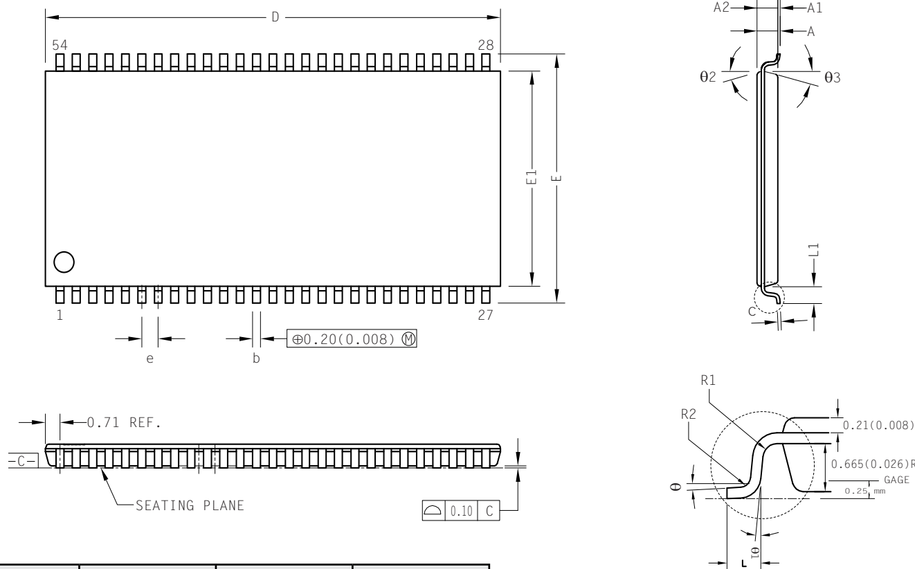
Figure 5.2 54-TSOP2
