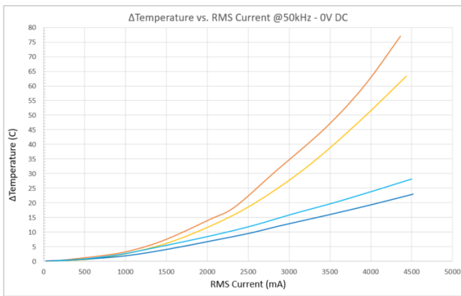
0V DC Bias
