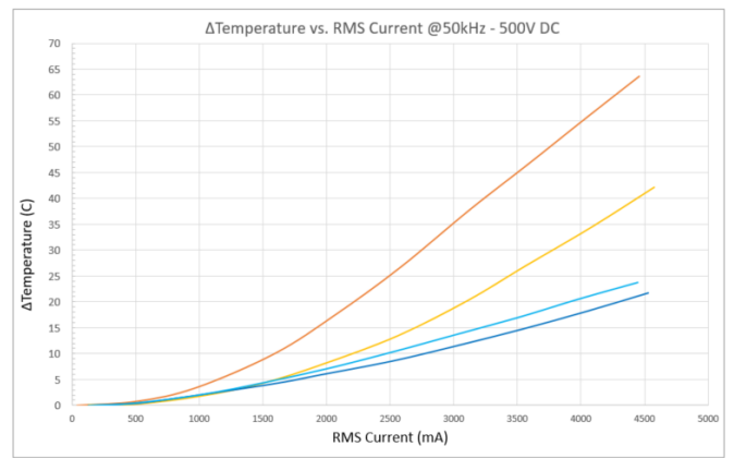
500V DC Bias
