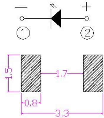
建议焊盘尺寸: Recommended Soldering Pattern
