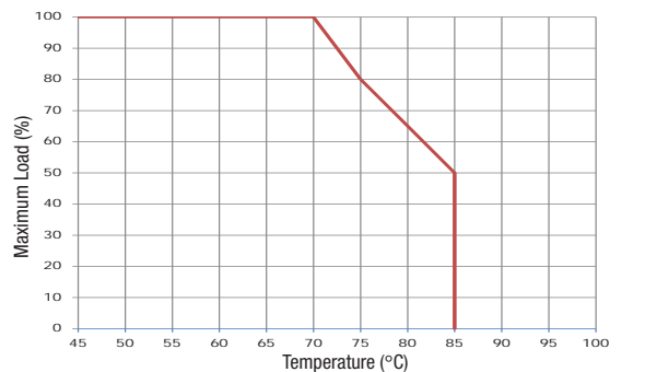
MTU2D1212MC
