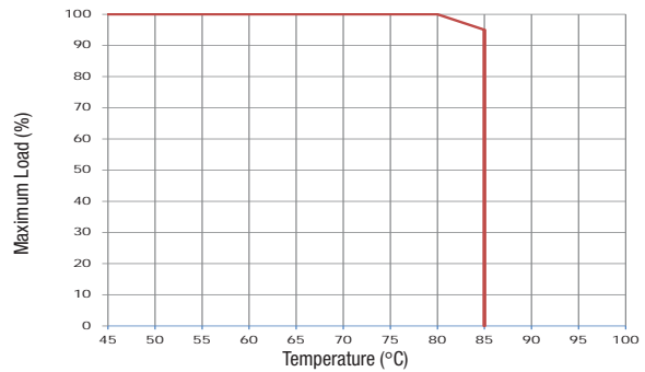
MTU2S1205MC
