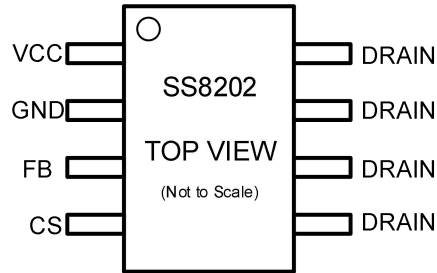
Figure 2. Pin Configuration
