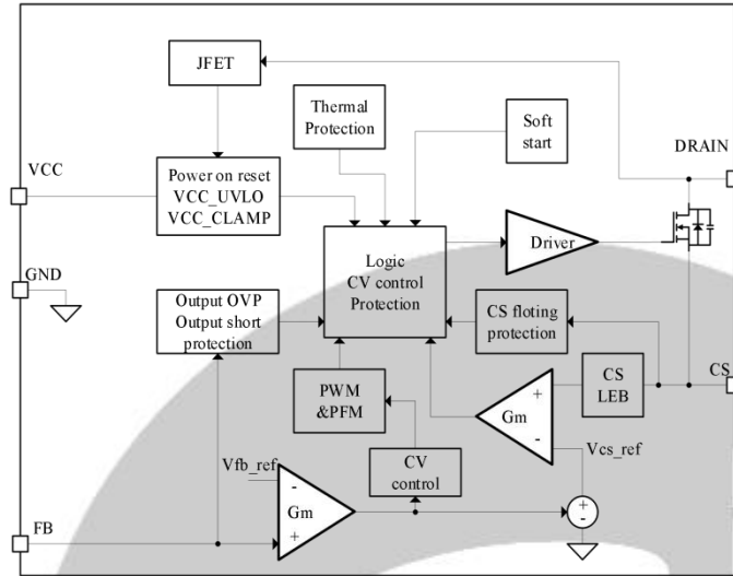
Figure 3. SS8202 Block Diagram
