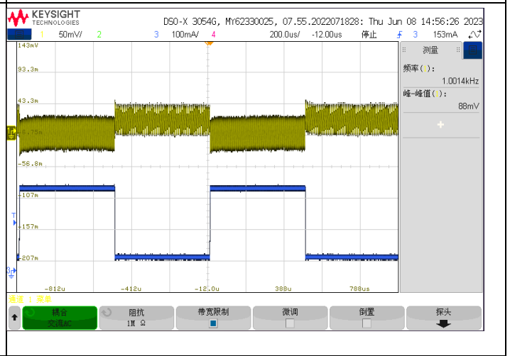
VINP =5V, VISO=3.3V, 动态负载电流: 30mA/270mA
