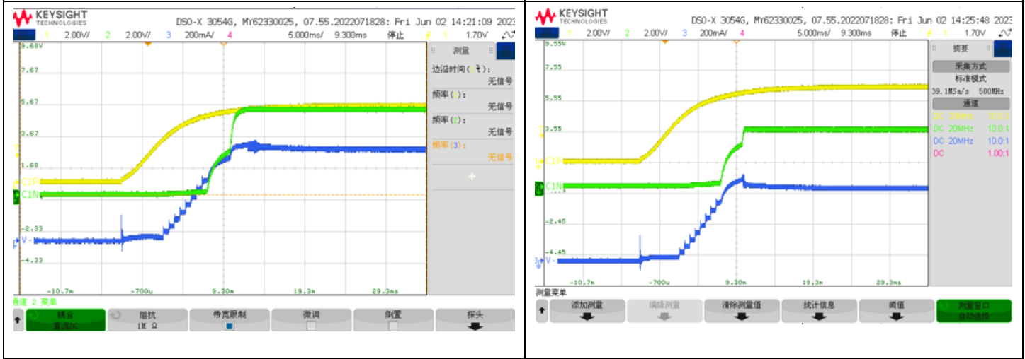
VINP=5V(黄色), VISO=5.4V(绿色), 软启动波形, IISO=300mA(蓝色)
