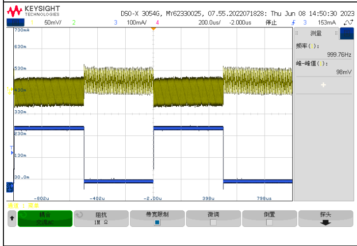
VINP =5V, VISO=5V, 动态负载电流: 30mA/270mA
