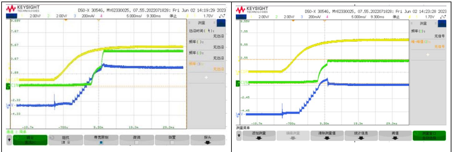
VINP=5V(黄色), VISO=5V(绿色), 软启动波形, IISO=300mA(蓝色)
